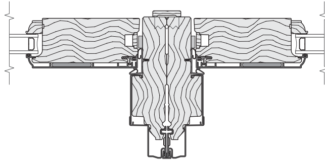
VERTICAL Combination (Joining) MULLION (Fixed Panels)
