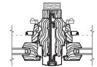
HH - Pella 1/2" x 4-9/16" Aluminum Reinforcement
