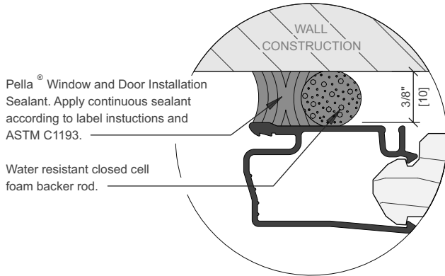
TYPICAL EXTERIOR PERIMETER SEALANT DETAIL
