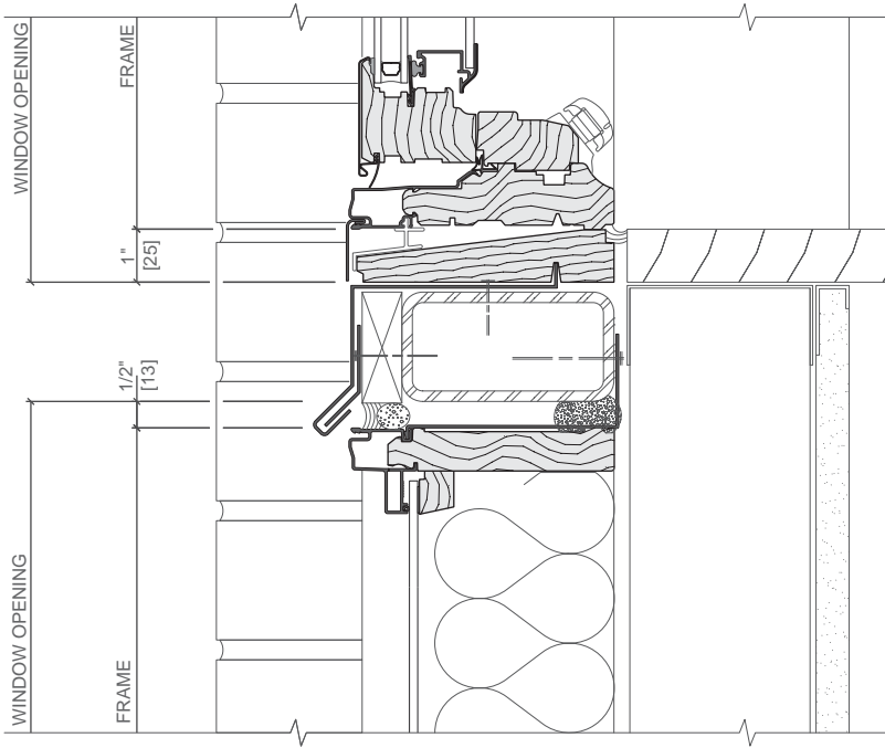
INTERMEDIATE SUPPORT DETAIL @ WINDOW SILL
