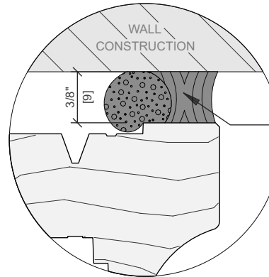
TYPICAL INTERIOR PERIMETER SEALANT DETAIL
