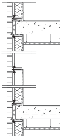
WALL SECTION
