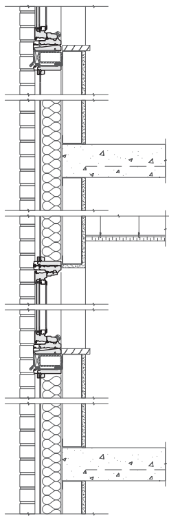
WALL SECTION
