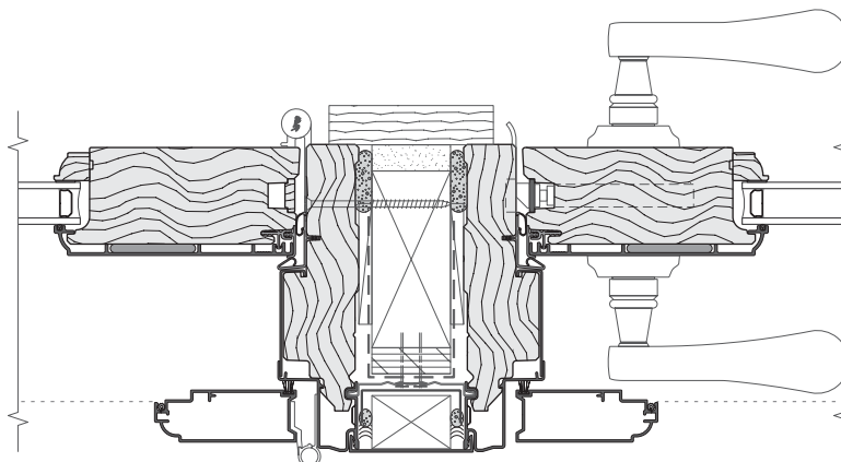
VERTICAL REINFORCING MULLION Operable Panels (lock Jamb/Hinge Jamb) Similar at lock jamb/lock jamb 2" mullion cover #72A9 with this structural mullion.
