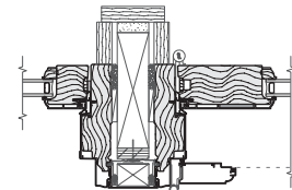
EE - 2 x 6 Wood
