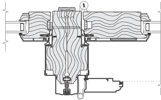
VERTICAL Combination (Joining) MULLION SIDELIGHT / HINGE JAMB (use 2" hinge screws) Similar at lock jamb and fixed jamb
