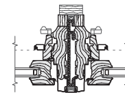
HH - Pella 1/2" x 4-9/16" Aluminum Reinforcement
