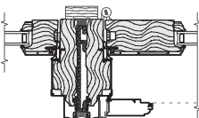
HH - Pella 1/2" x 4-9/16" Aluminum Reinforcement
