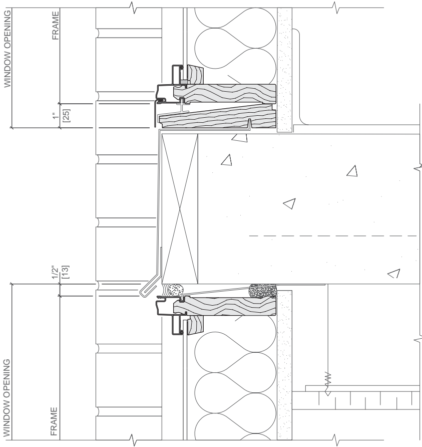
INTERMEDIATE SUPPORT DETAIL ON FLOOR SLAB
