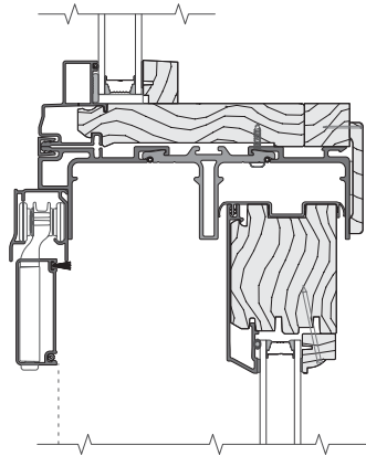
HORIZONTAL JOINING MULLION TRANSOM / RESERVE SLIDING DOOR (VENT)
