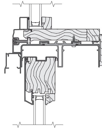
HORIZONTAL JOINING MULLION TRANSOM / RESERVE SLIDING DOOR (FIXED)
