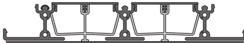
1-1/2" Weep Sill
