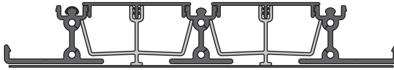
1-1/2" Weep Sill
