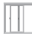
Sliding Window
