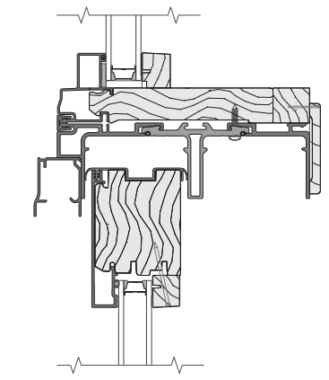
HORIZONTAL JOINING MULLION TRANSOM / SLIDING DOOR (FIXED)
