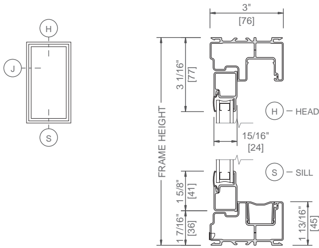
BLOCK FRAME
