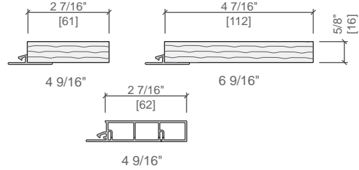
Optional Factory Applied Jamb Extensions
