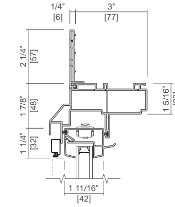
Double Wall Flush Flange
