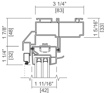
1" Triple IG
