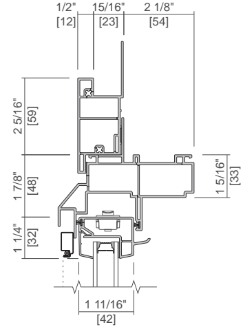
Standard Fin with Flat Casing
