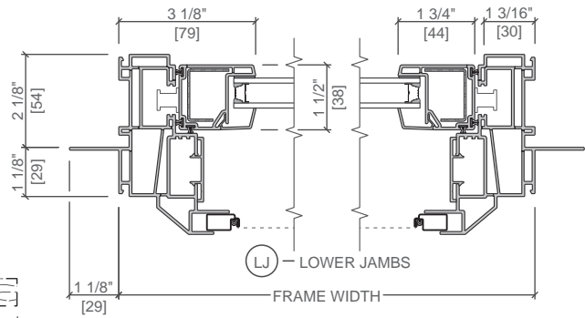
Optional Factory Applied Jamb Extensions
