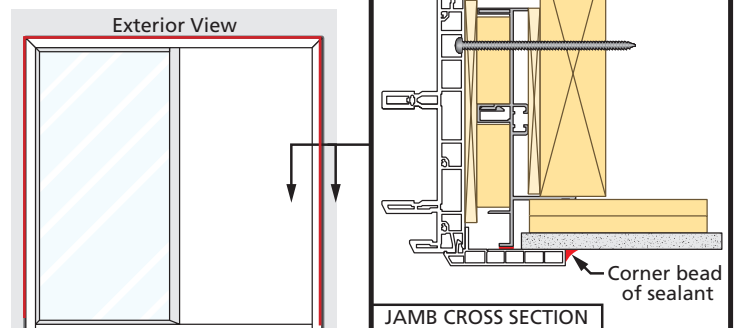
Flush Flange Doors
