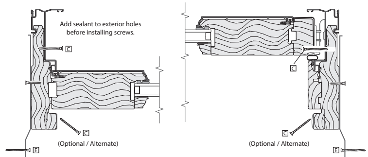
Clip/Screw, Jamb
