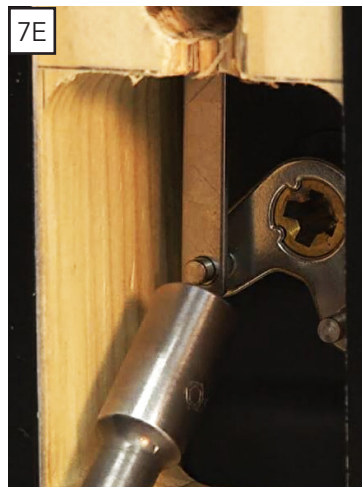
Retaining washer
