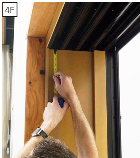
Marking for pilot hole location
