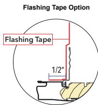
Flashing Tape Option
