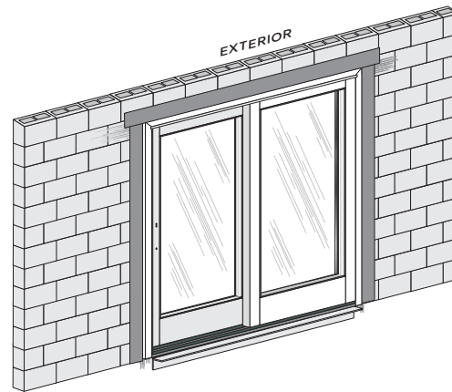
Fin to Frame Seal Flashing Tape Option
