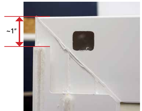
Interior view - top corner of interlocker panel
