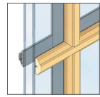
Simulated-Divided-Light without Spacer 7/8" 1
